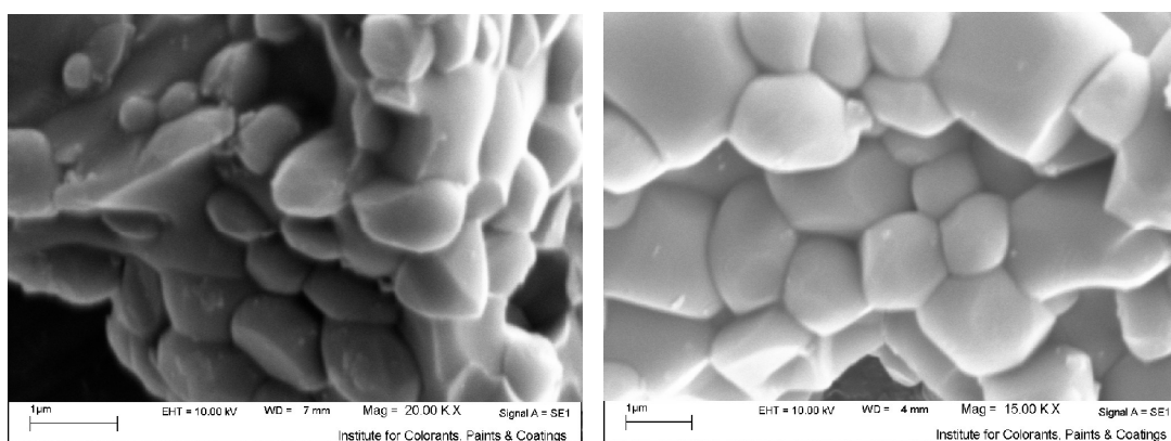
Fig. 6. SEM image of sol-gel derived ATM in 1300°C (left) and 1350°C (right) for 3h.
