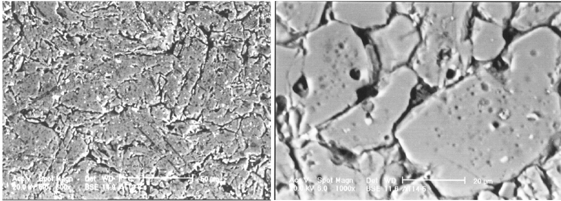
Fig. 2. SEM image of solid-state derived AT in 1350 °C (left) and 1450 °C (right) for 4h.
