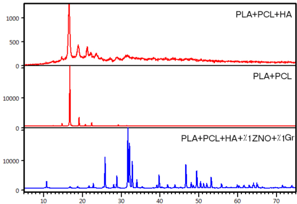
Fig. 5. The XRD patterns of PLA-PCL, PLA-PCL-HA, and PLA-PCL-HA-ZnO-Gr nanoparticles.
