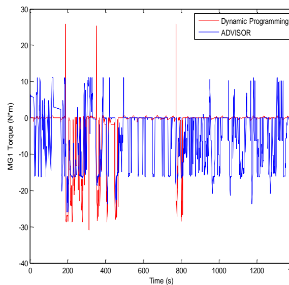
Figure 8: MG1 torque
