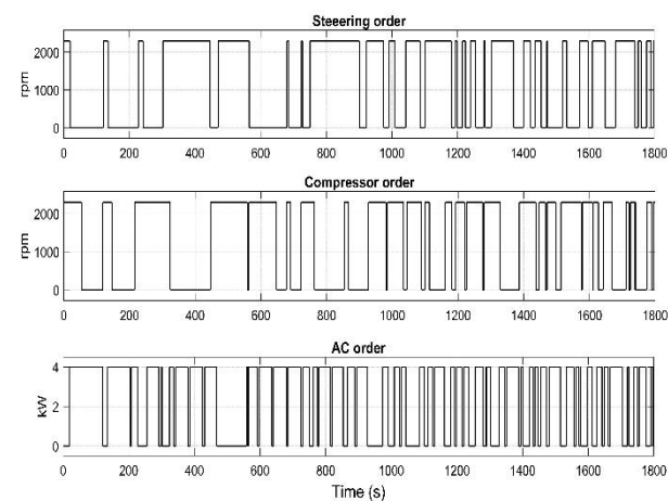
Figure 19: Final commands sent to the accessories
