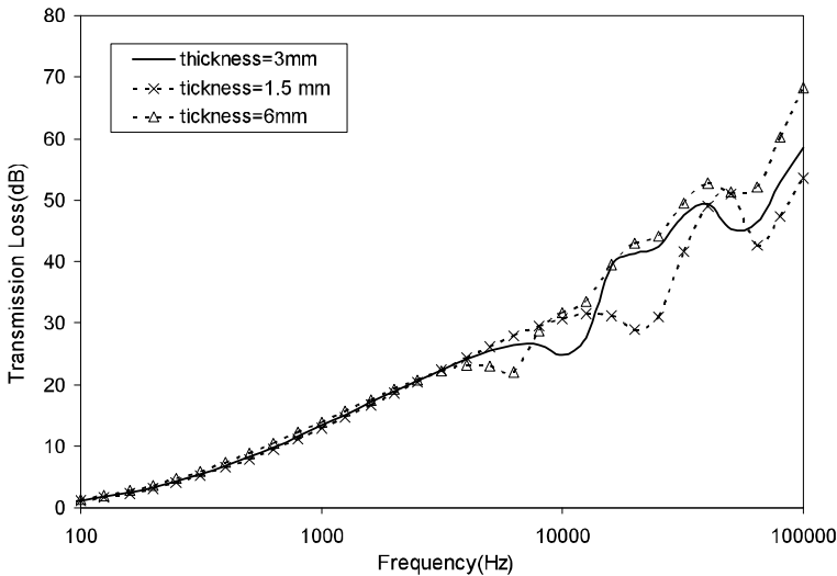
Fig. 13. Comparison of TL for the structures with different thicknesses of foam
