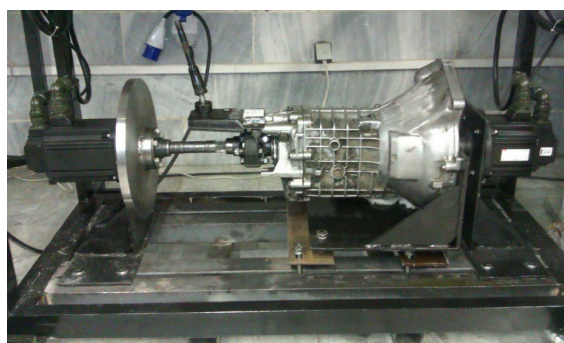
Fig. 7. Platform section of the sub-scale simulator
