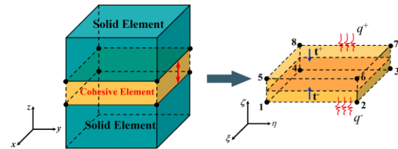
Figure 10 8-node zero-thickness cohesive element [54].
