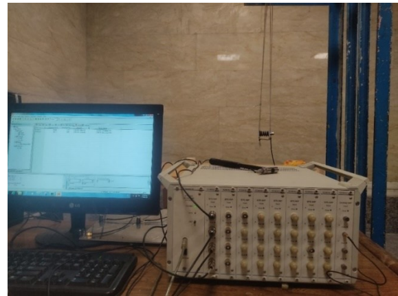
Figure 10: Structural Configuration during Modal Testing
