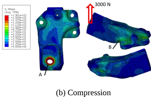
Figure 4. Finite element modeling of the part.
