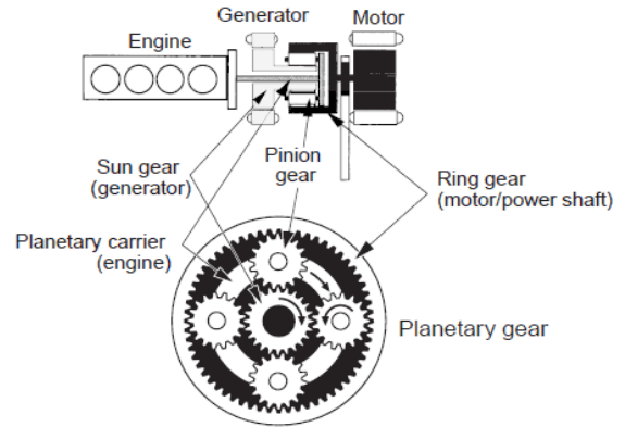
Figure 3: power split device [16]
