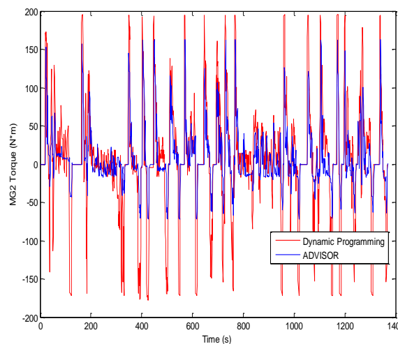
Figure 7: MG2 torque
