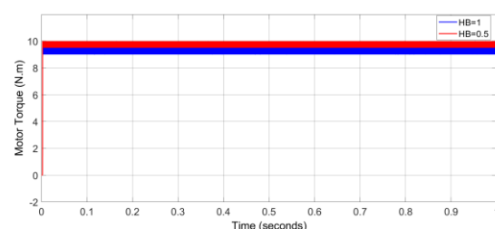
Figure 7: Effect of Hysteresis Bandwidth Variation on output Torque.
