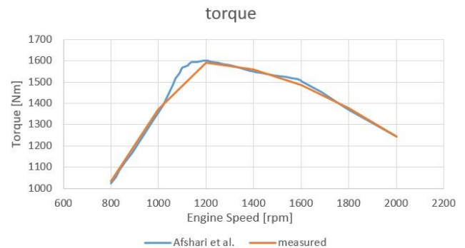
Figure 3: torque comparison of Afshari et al.[18]'s study with present study for OM457
