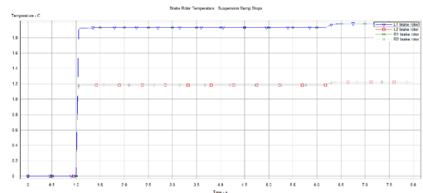
Figure33: Brake Rotor Temperature C-Time(s) “ABS_OFF”
