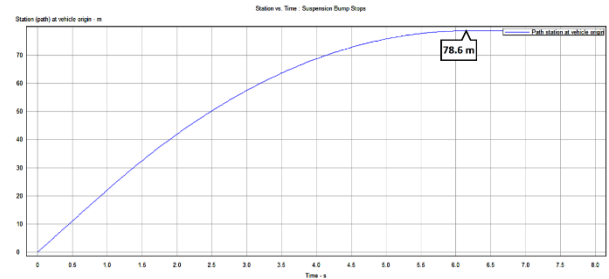
Figure32: Brake Distance m-Time(s) “Carsim_ABS_OFF”
