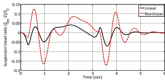
Figure 14. Suspension travel ratio, middle suspension
