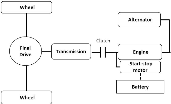
Fig2. Start-stop (SS)
