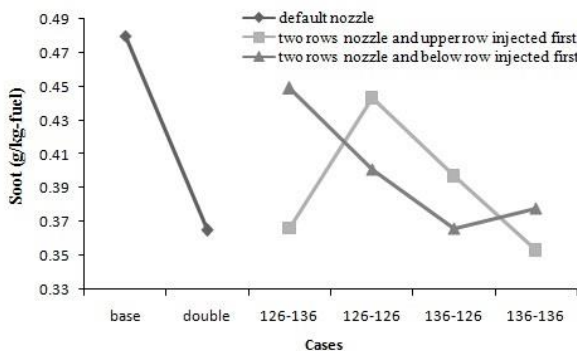
Fig 13. Soot emission
