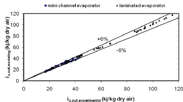
Fig. 11. Comparison of modeling and experimental evaporator outlet air enthalpy for mini-channel and laminated evaporators
